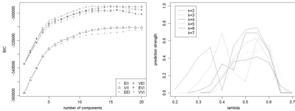
Fig. 4. BIC and prediction strength to estimate K and \lambda .
